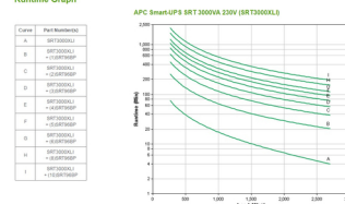
Runtime Graph
